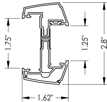
IMPACT LITE FRAME ALUMINUM
