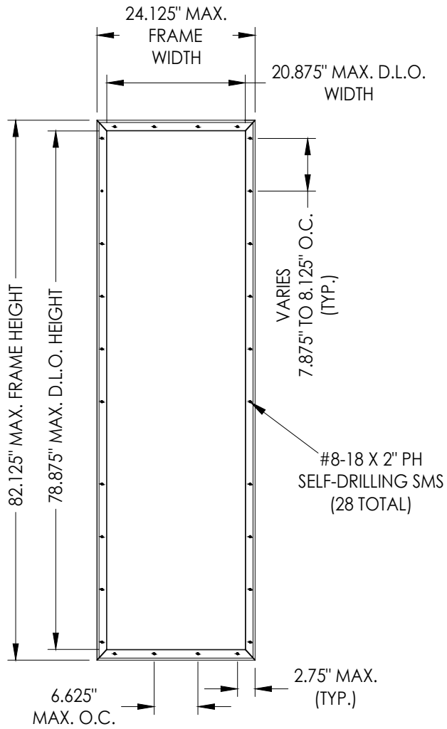
ALUMINUM IMPACT LITE FRAME 8'-0" DOOR/SIDELITE
