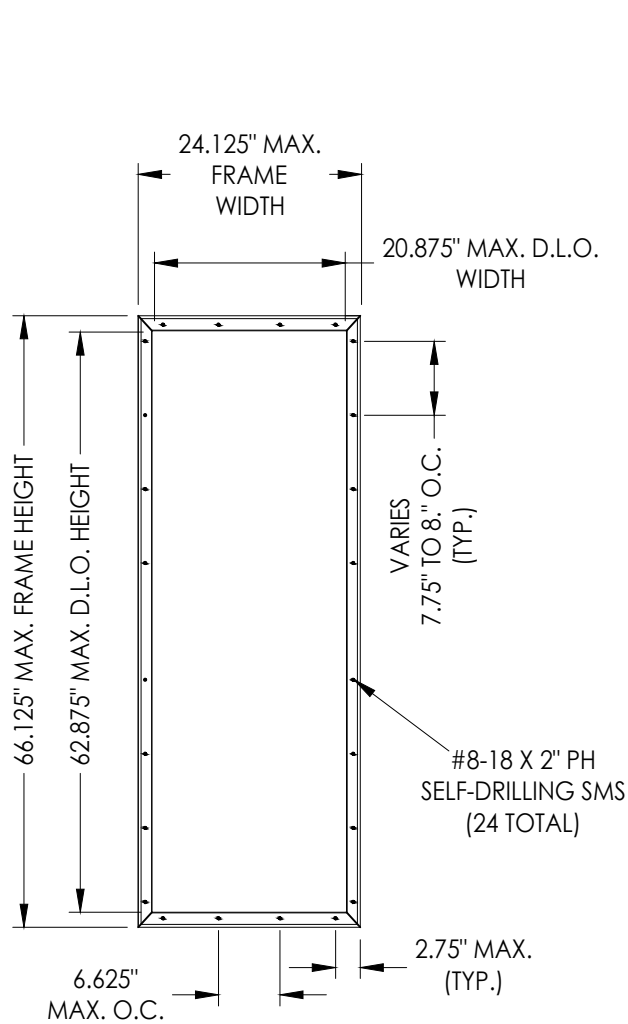
ALUMINUM IMPACT LITE FRAME 6'-8" DOOR/SIDELITE
