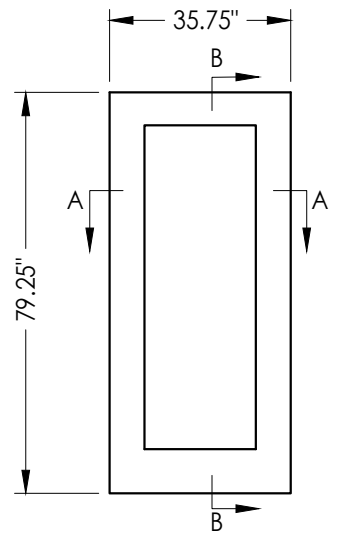
FIBERGLASS DOOR PANEL Plastpro 6'-8"
